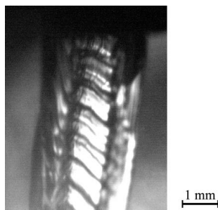
Figure 4.20: A stroboscopic image of liquid screen generated using a splash plate setup. The screen is agitated at a frequency of 20 kHz, showing controlled thickness variations in the middle of the screen. The thicker outer edges remain virtually unaffected.
