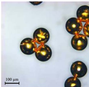
(a) Monodisperse Feingold droplets \phi 120 \mu\text{m} .
