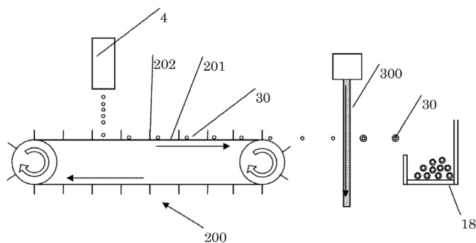
Figure 4.21: Multi component particle generating system, particle based [29]. Linear configuration: Powder particles are deposited on a conveyor belt (200) by dispenser 4. The particles (30) are subsequently thrown through liquid screen 300 creating encapsulates which are collected in gutter 18. A further in-depth description of all noted numbers can be found in the patent application.
