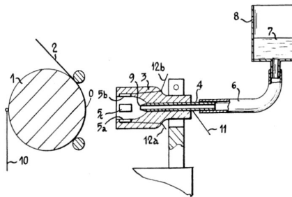
Figure B.6: Electrostatic pull inkjet; Paillard S.A., 1962 [119].
