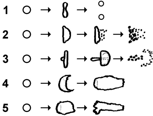
Figure 3.15: Droplet deformation and breakup occurring with increased We numbers [62].
