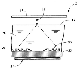
Figure B.12: Focused acoustic beam ejection with Fresnel lens; Xerox Corporation, 1991 [131].
